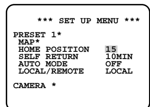
Setup menu
