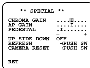
Special menu
