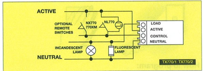
Fig 2. Wiring diagram for combination of incandescent and fluorescent loads
