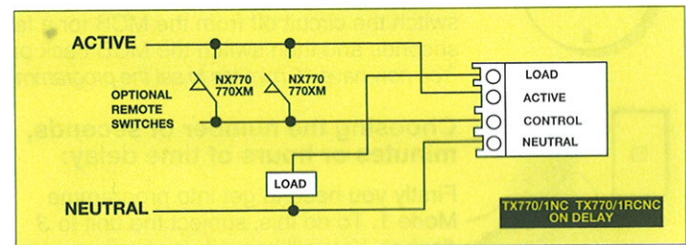
Fig 4. Turning load 'off' for timer period (Normally closed - NC Timer).
