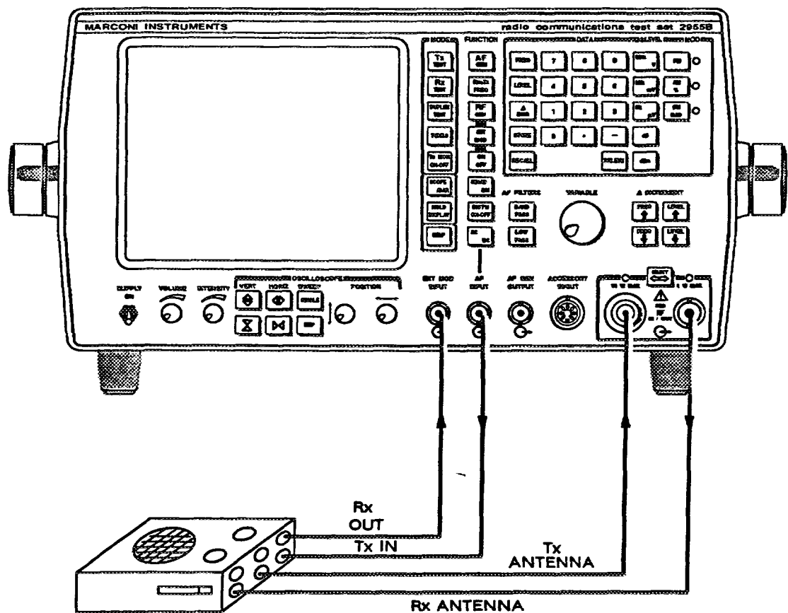
Two-port connections
